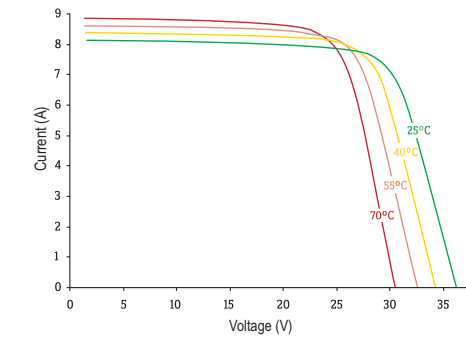
SLK60P6L - 225W I-V characteristics with a variety of cell temperatures at 92.94 W/m 2 (1,000 W/m 2 )
