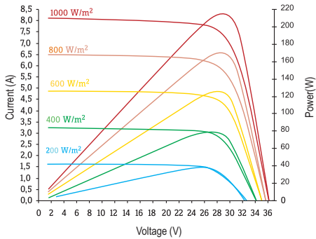
SLK60P6L - 225W I-V and Pmax characteristics with a variety of radiation levels at 77°F (25°C)
